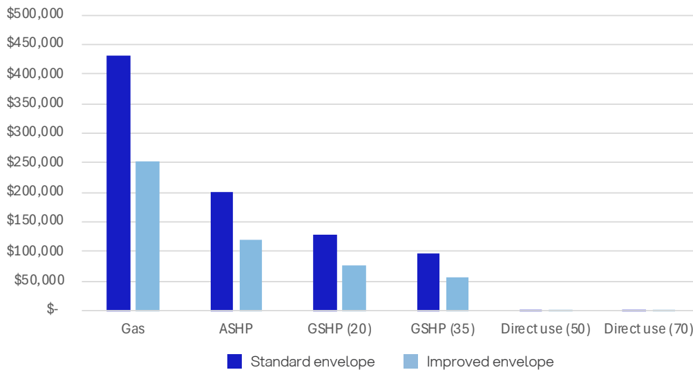
Figure 1: This graph shows the impact of smart building design on energy required for the operation of a greenhouses, comparing thermally insulated material (light blue) and traditional building material (blue). Large savings in energy costs can be achieved by investing in improved building material.
