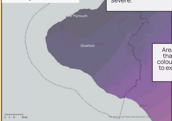
10 % probability of exceedance in 50 years PGA map
