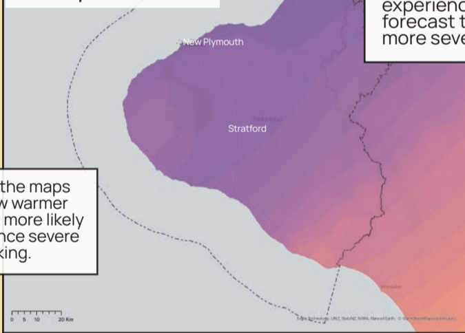
2 % probability of exceedance in 50 years PGA map
