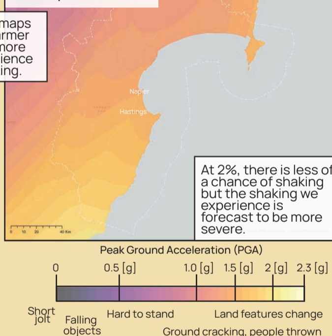
2 % probability of exceedance in 50 years PGA map
